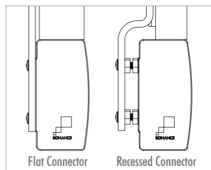
Mounting Option 1: Bracket Wall Mount
